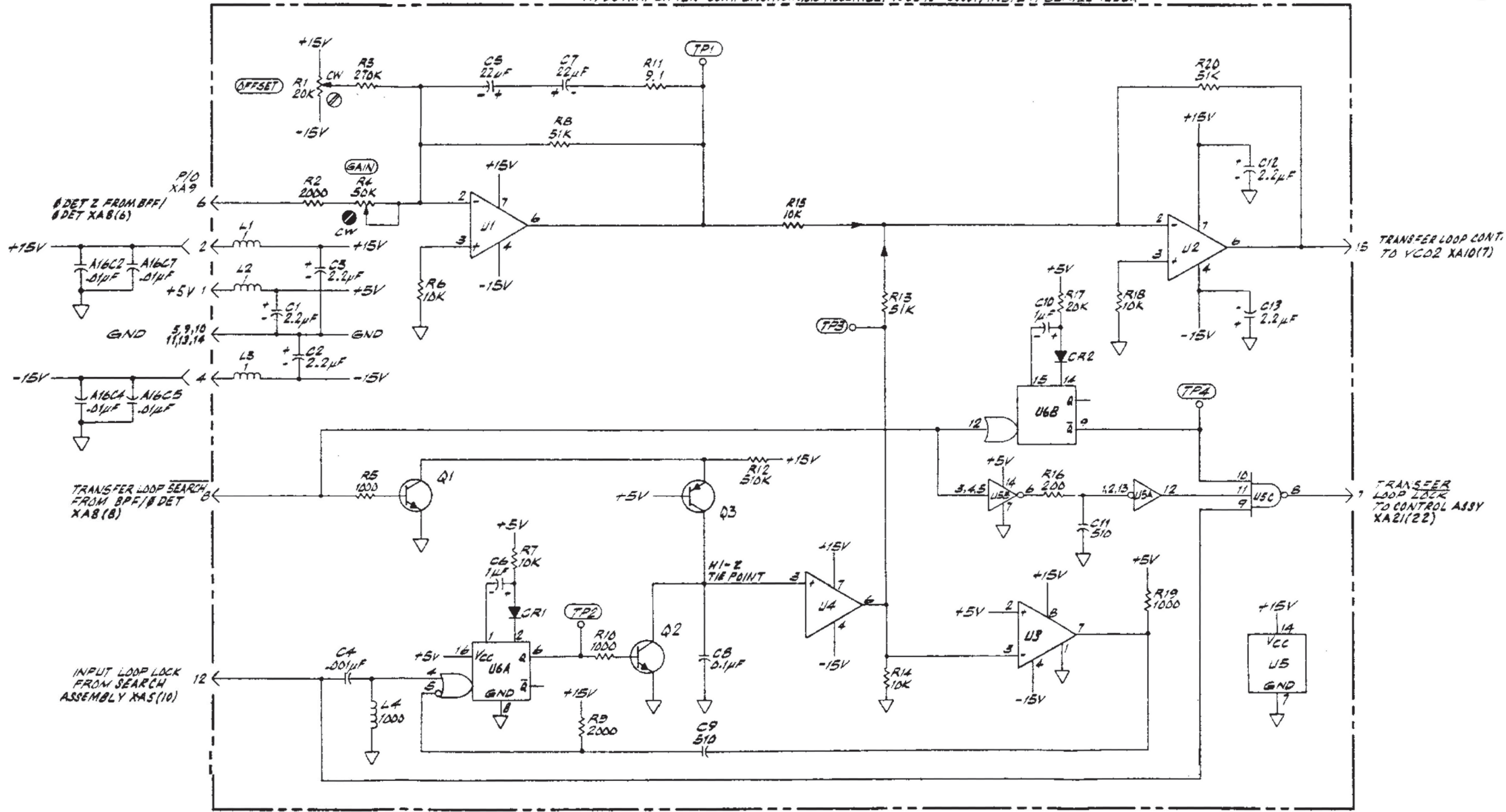
Figure 8-15. A9 DC Amplifier/Compensator No. 2 Assembly
