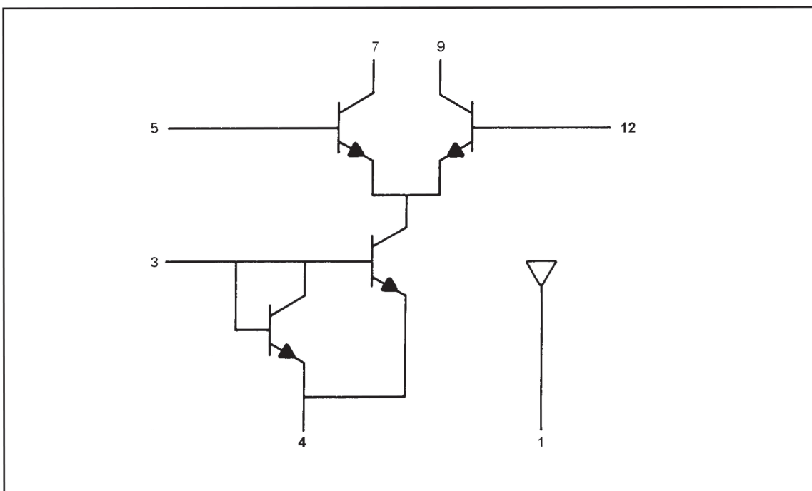
Figure 4-44. Transistor Array 1858-0018
