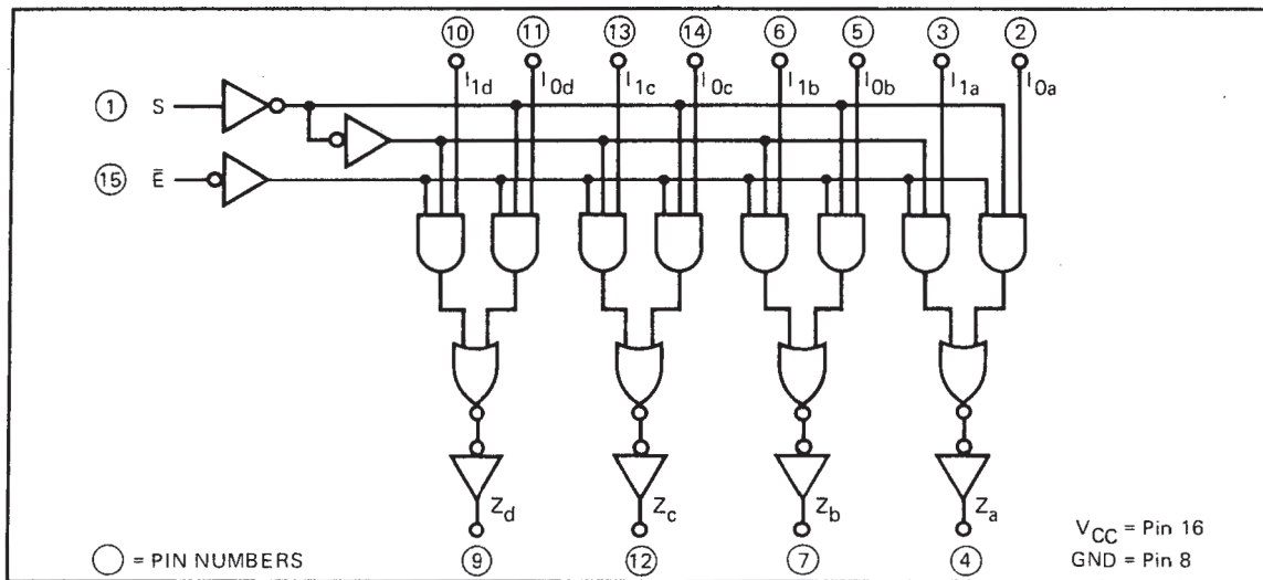
Figure 4-24. Quad 2-Input Multiplexer 1820-0616
