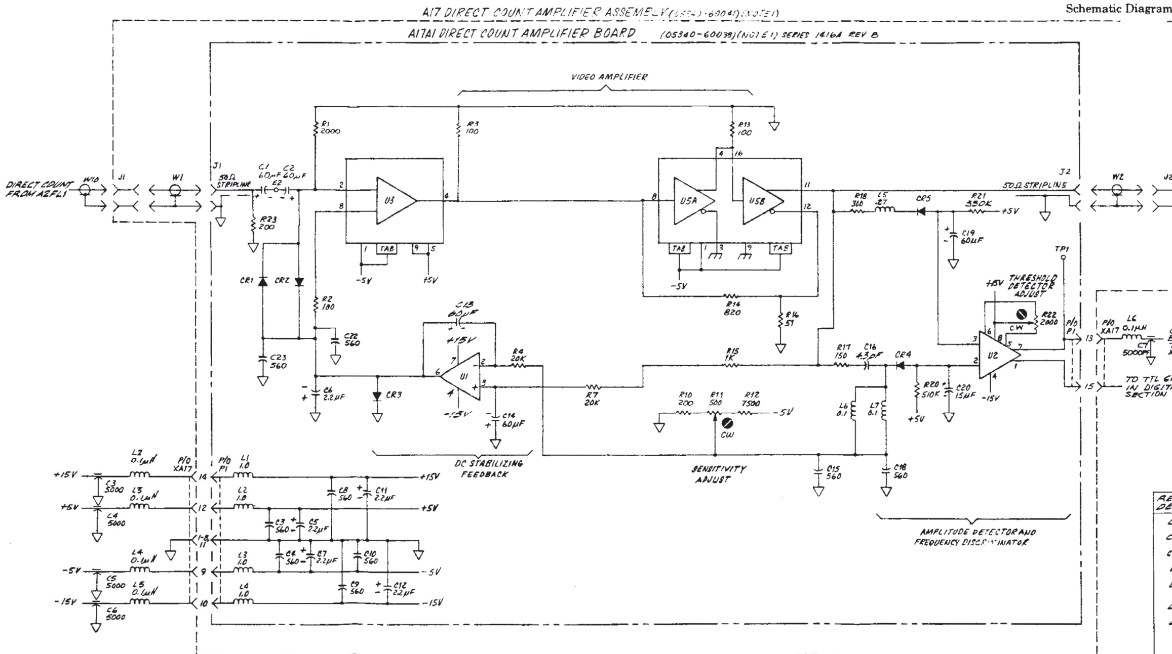
Figure 8-23. A17 Direct Count Amplifier Assembly
