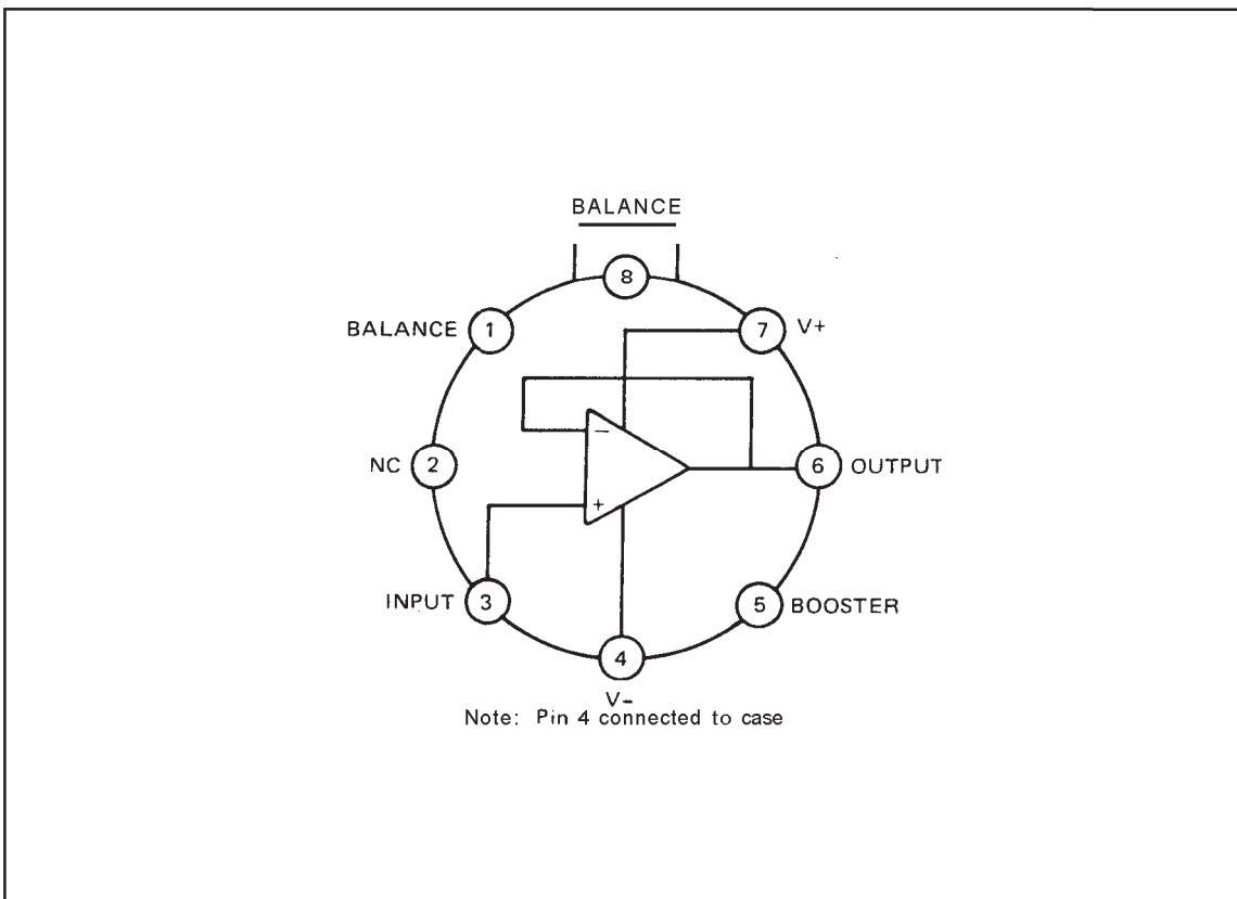
Figure 4-40. Operational Amplifier 1826-0021
