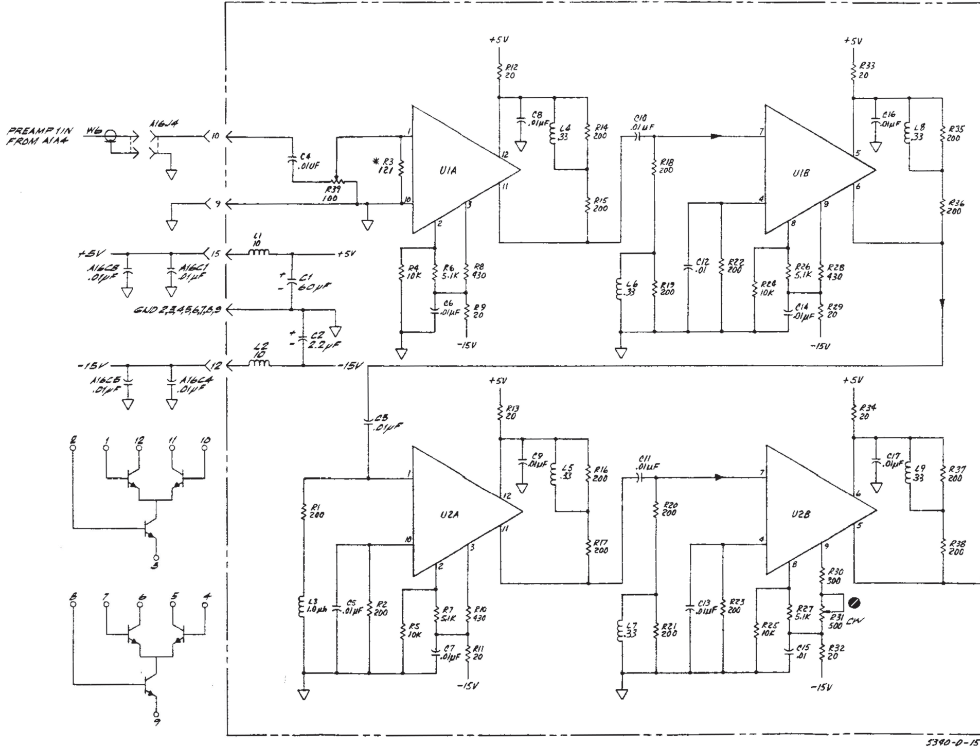
Figure 8-19. A13 Limiter/Amplifier Assembly
