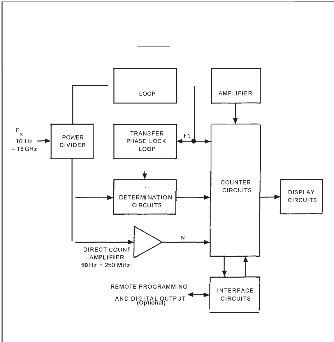
Figure 4-45. Simplified Block Diagram
