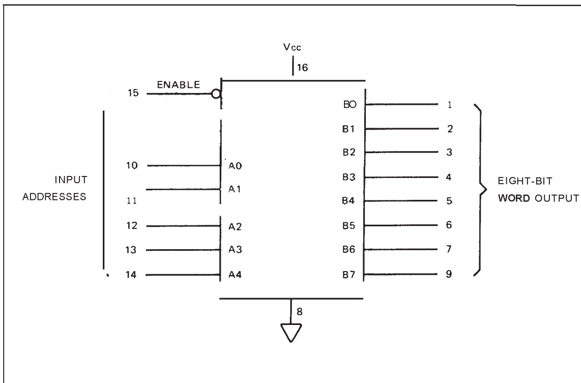
Figure 4-3. Logic Diagram for 1816-0003,1816-0004,1816-0184,and 1816-0185ROM's
