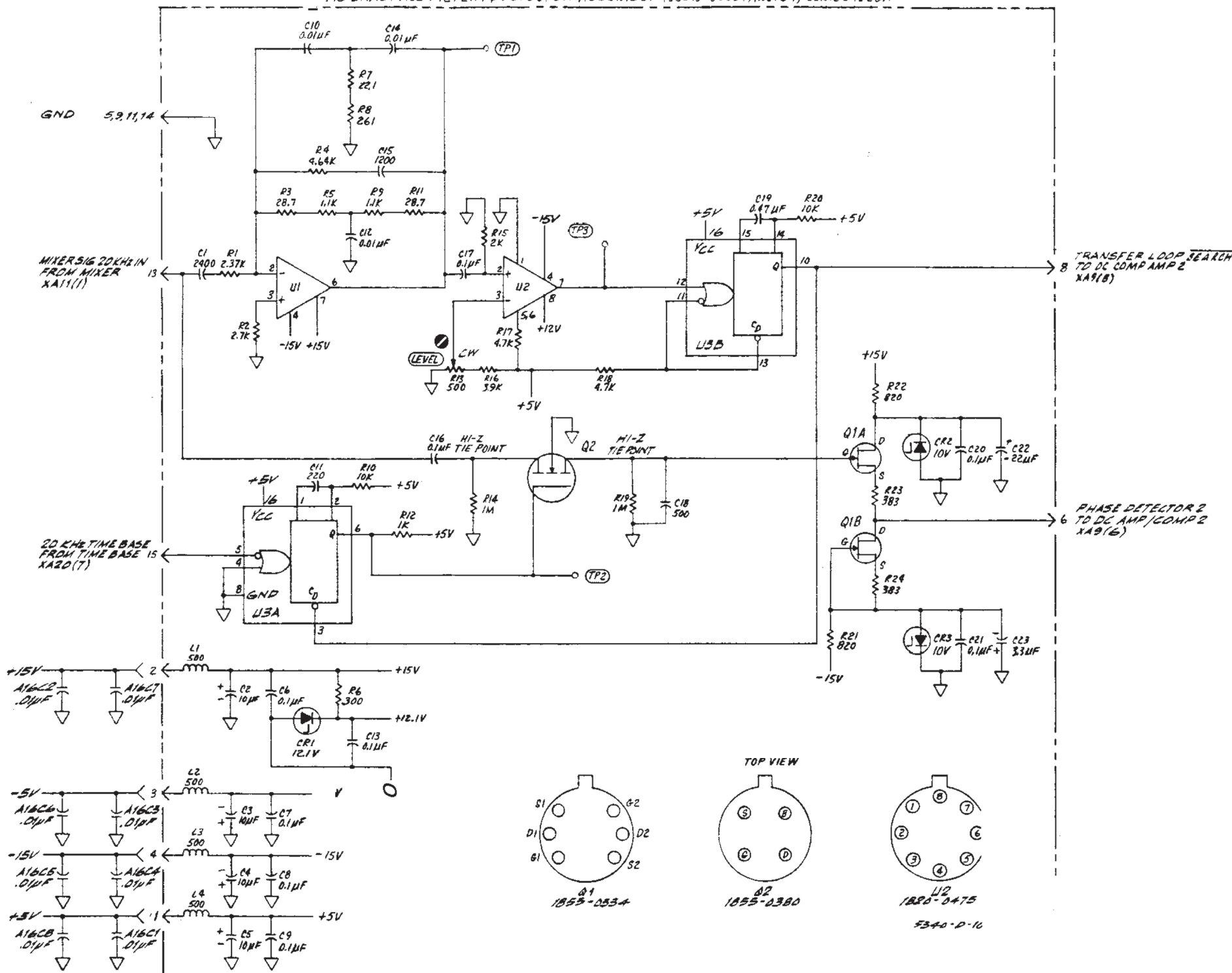
Figure 8-14. A8 Bandpass Filters/φ Detector Assembly
