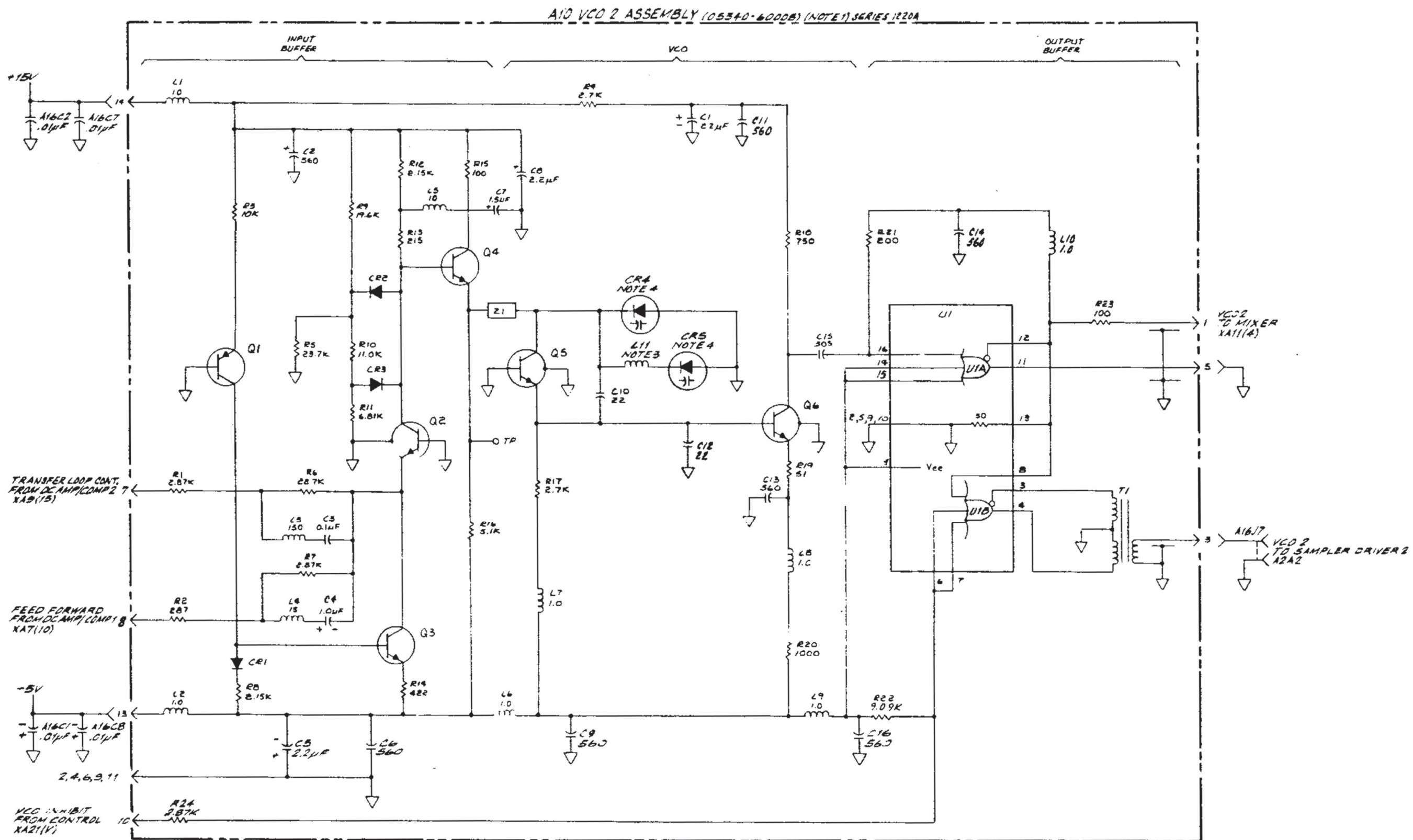
Figure 7-6. A10 VCO No. 2 Assembly (Series 1220A), Schematic Diagram
