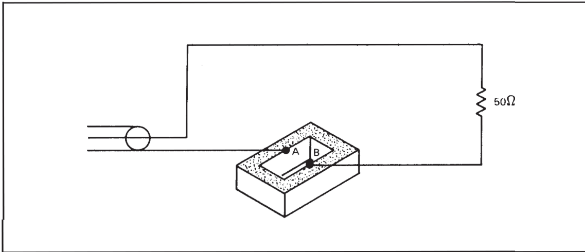
Figure 4-48. Sampler Slot
