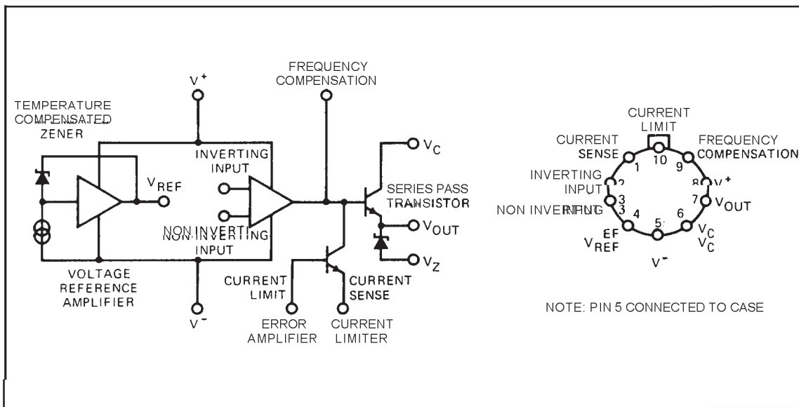
Figure 4-38. Voltage Regulator 1826-0010
