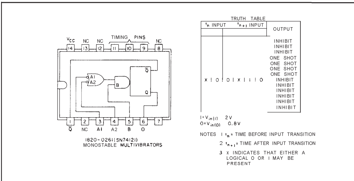
Figure 4-11. Monostable Multivibrator 1820-0261
