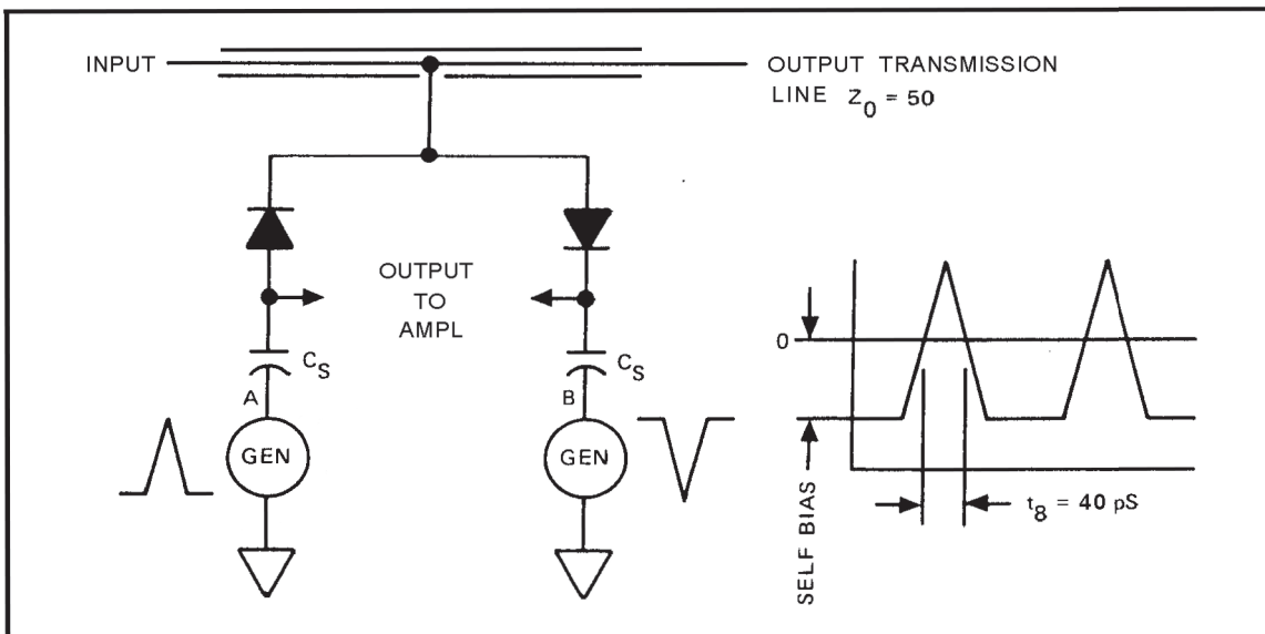
Figure 4-47. Balanced Sampler
