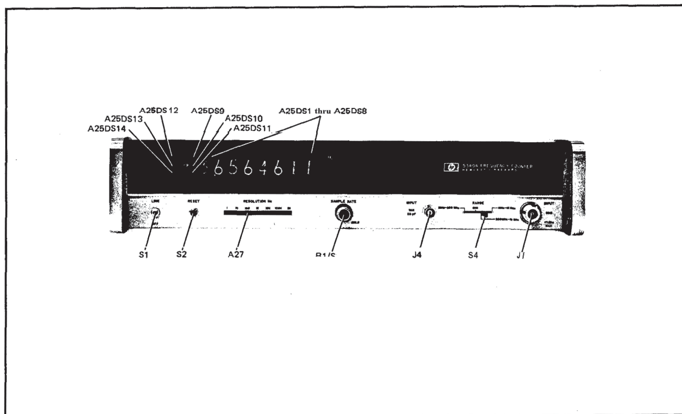
Figure 8-4. 5340A Front Panel Reference Designations
