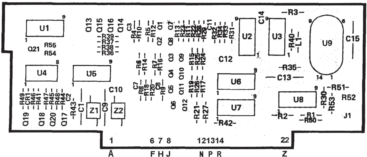
Figure 7-1. A2 Component Locator Series 1236A
