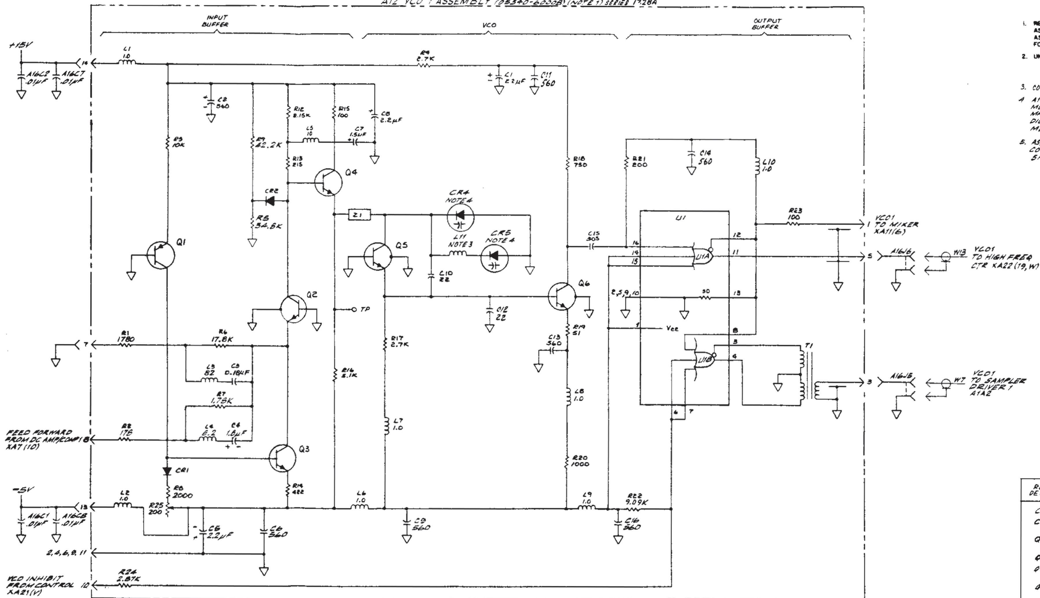
Figure 8-18. A12 VCO No. 1
