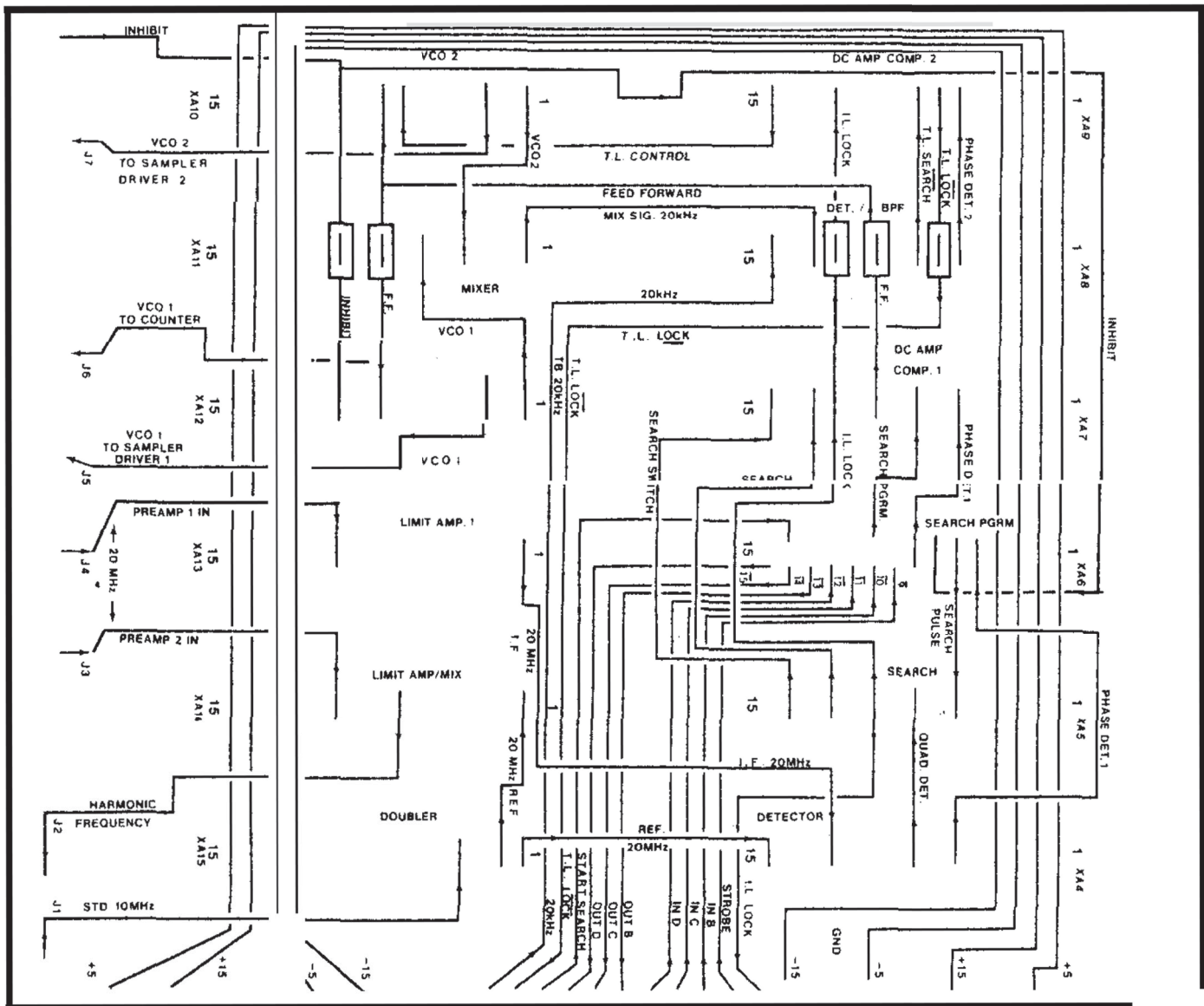
Figure 8-22. A16 Casting Motherboard
