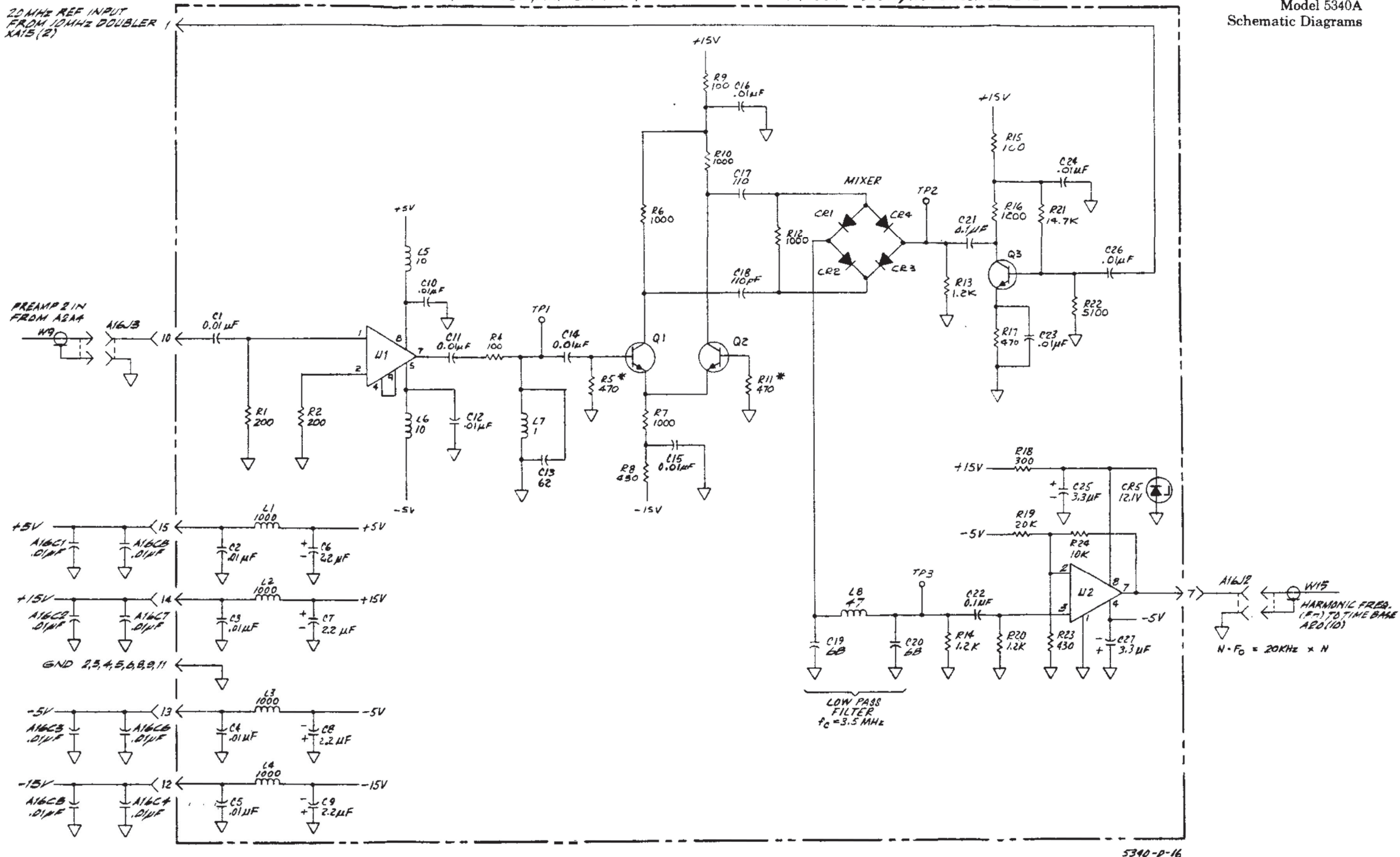
Figure 8-20. A14 Limiter/Amplifier/Mixer Assembly
