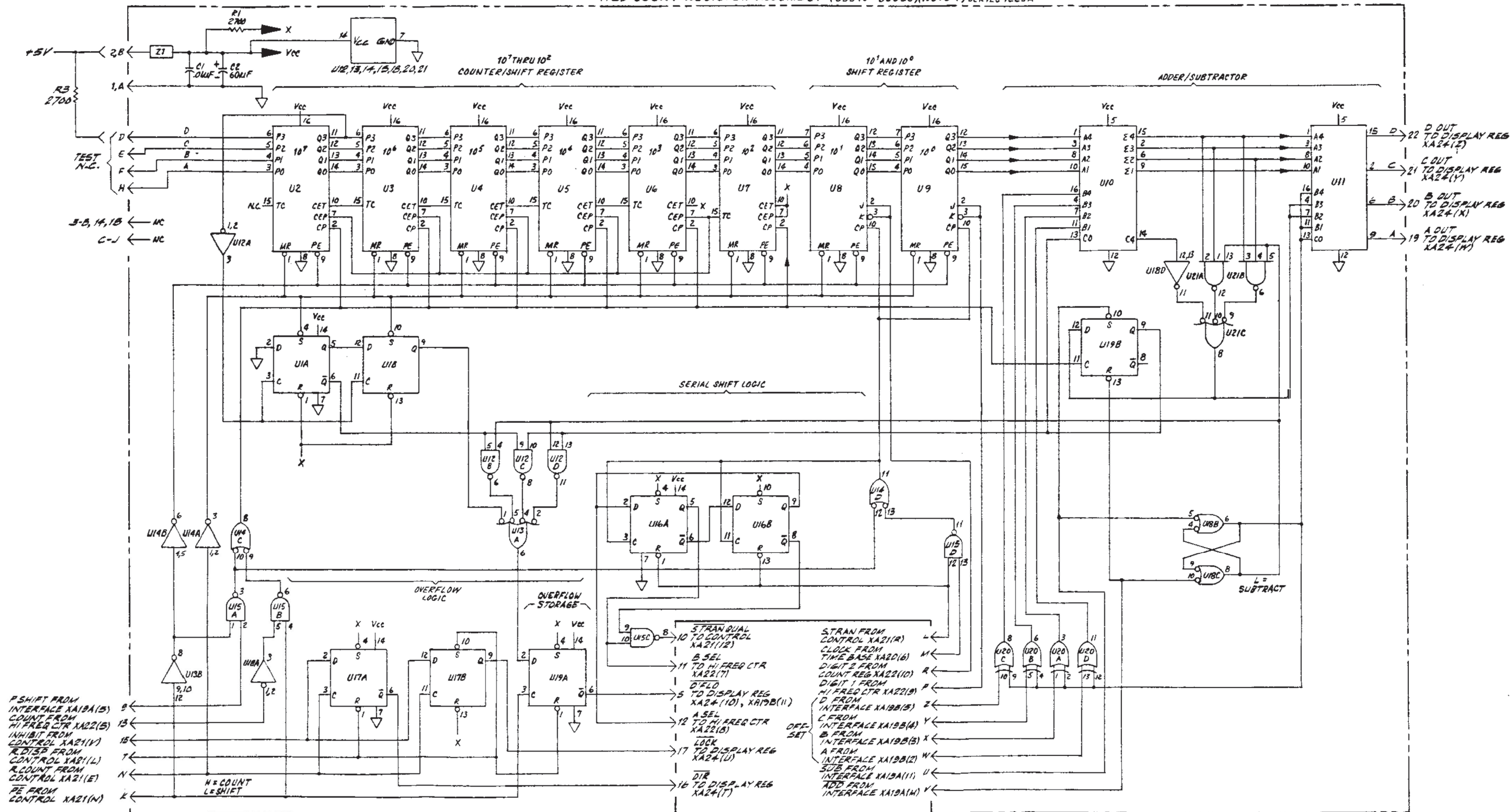
Figure 8-30. A23 Count Register Assembly
