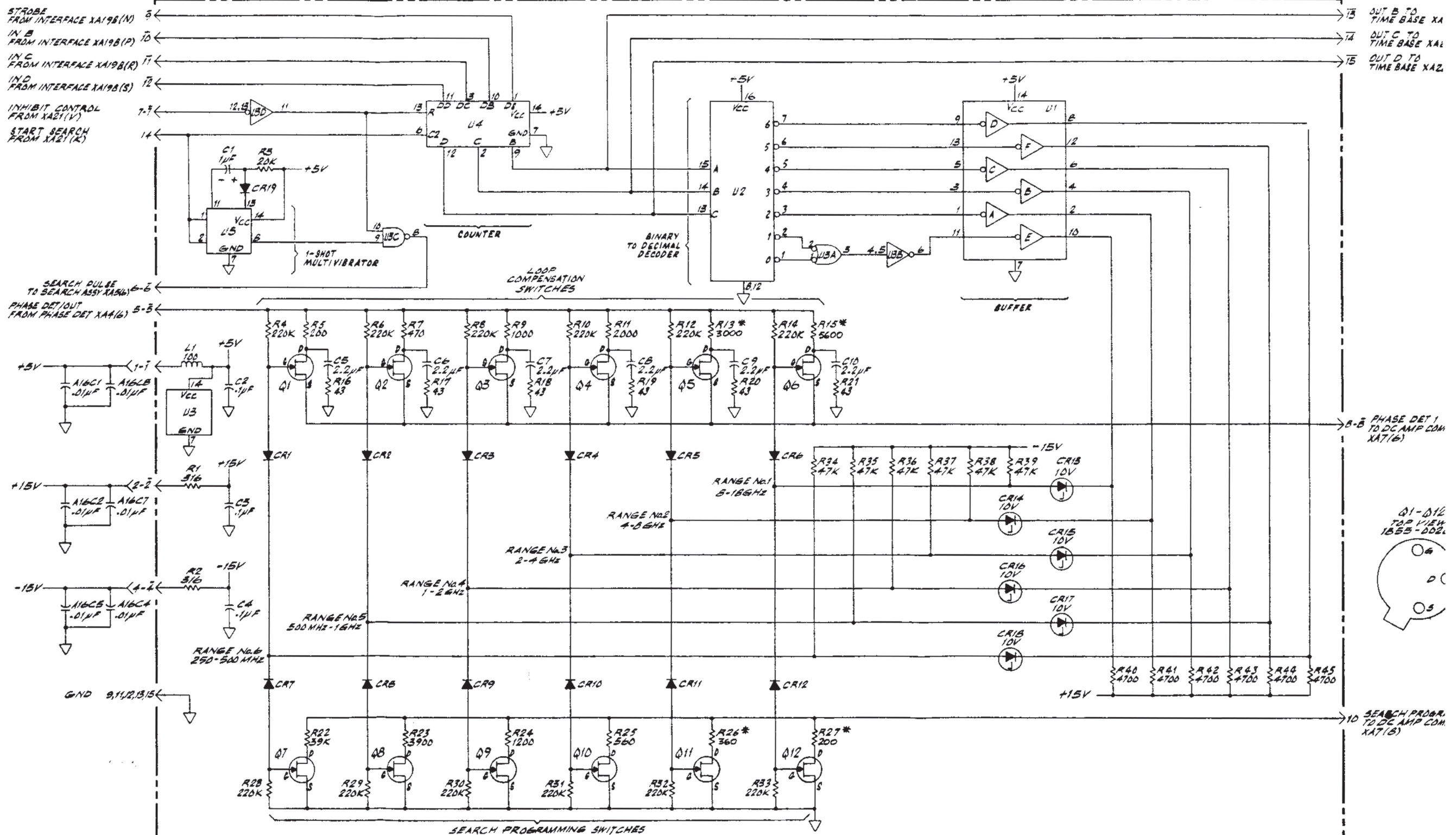
Figure 8-12. A6 Search Programmer Asse
