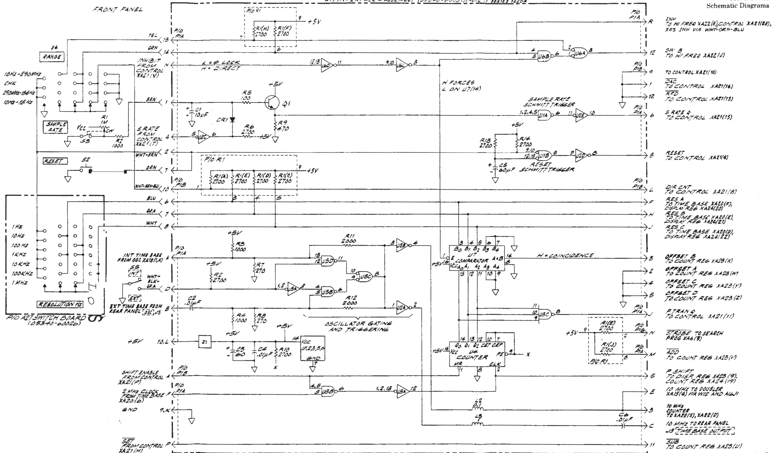
Figure 8-25. A19 Interface A Assembly (Standard Instrument), A27 Resolution Switch Assembly
