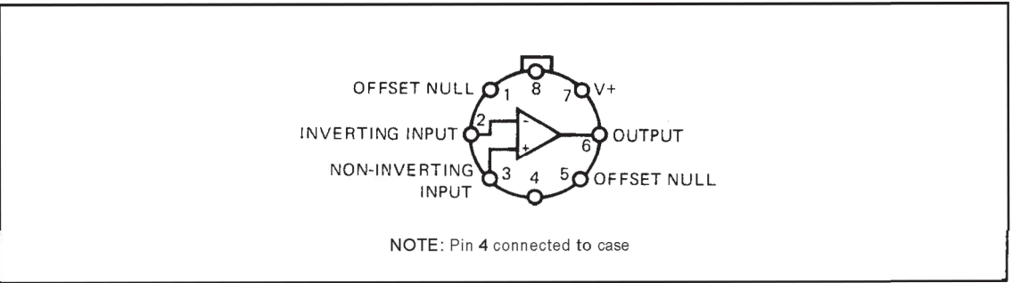
Figure 4-10. Operational Amplifier 1820-0216
