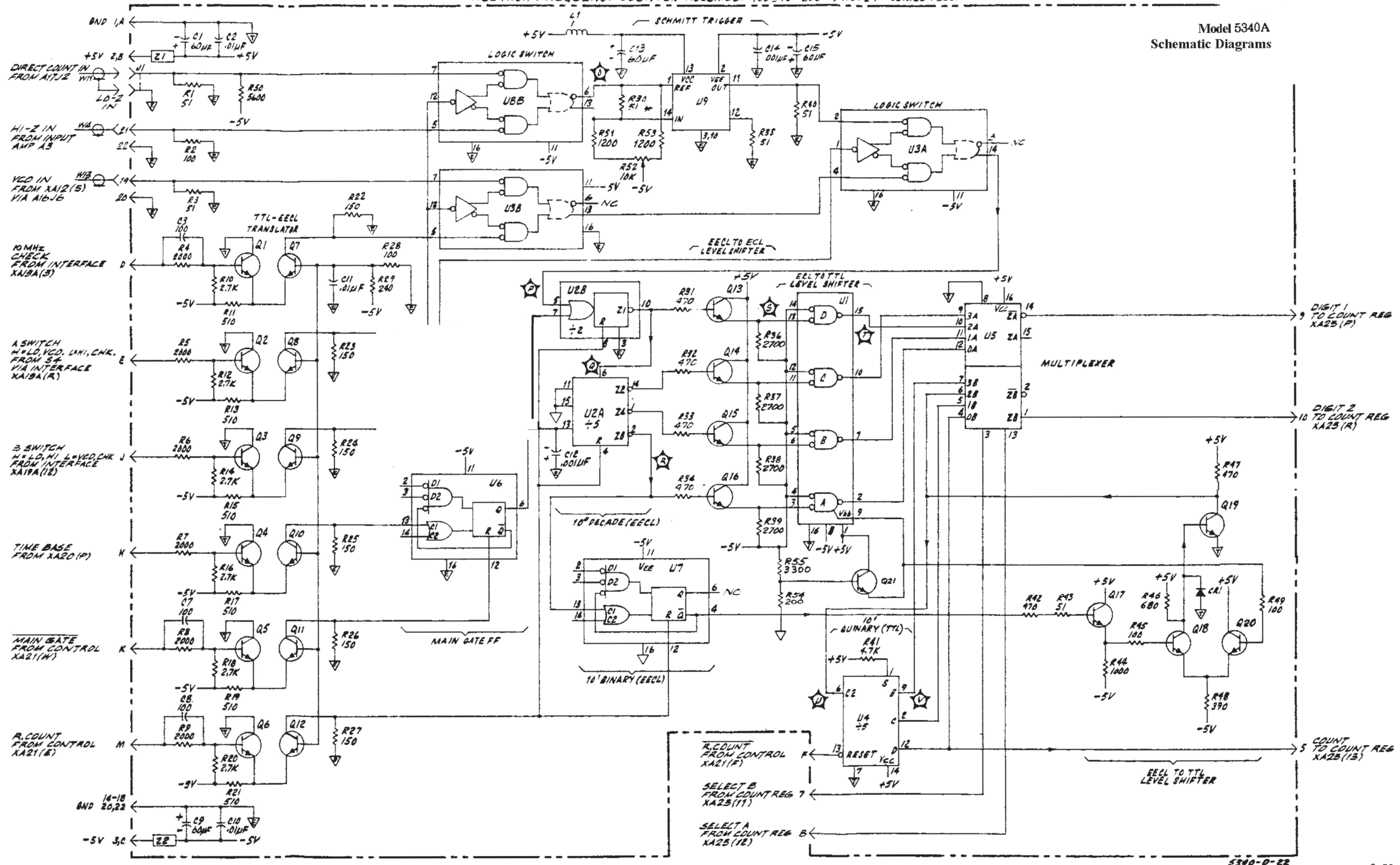
Figure 8-29. A22 High Frequency Counter Assembly
