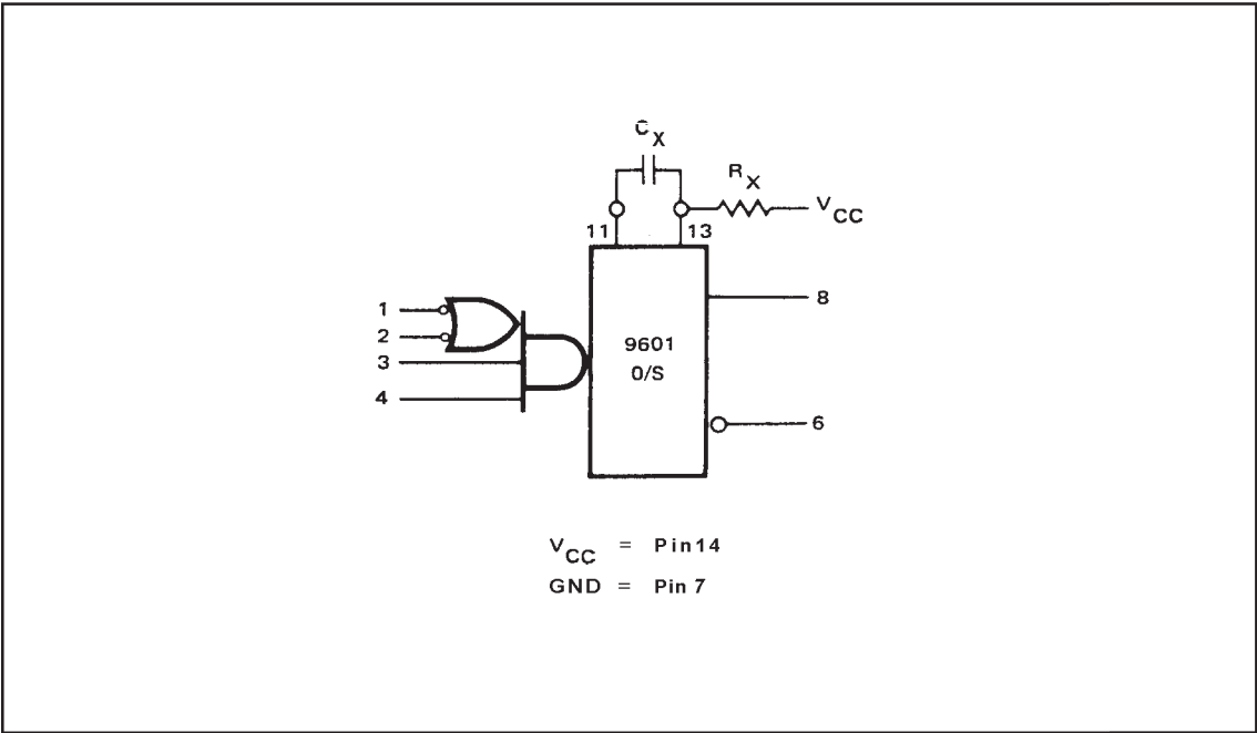
Figure 4-8. Monostable Multivibrator 1820-0207
