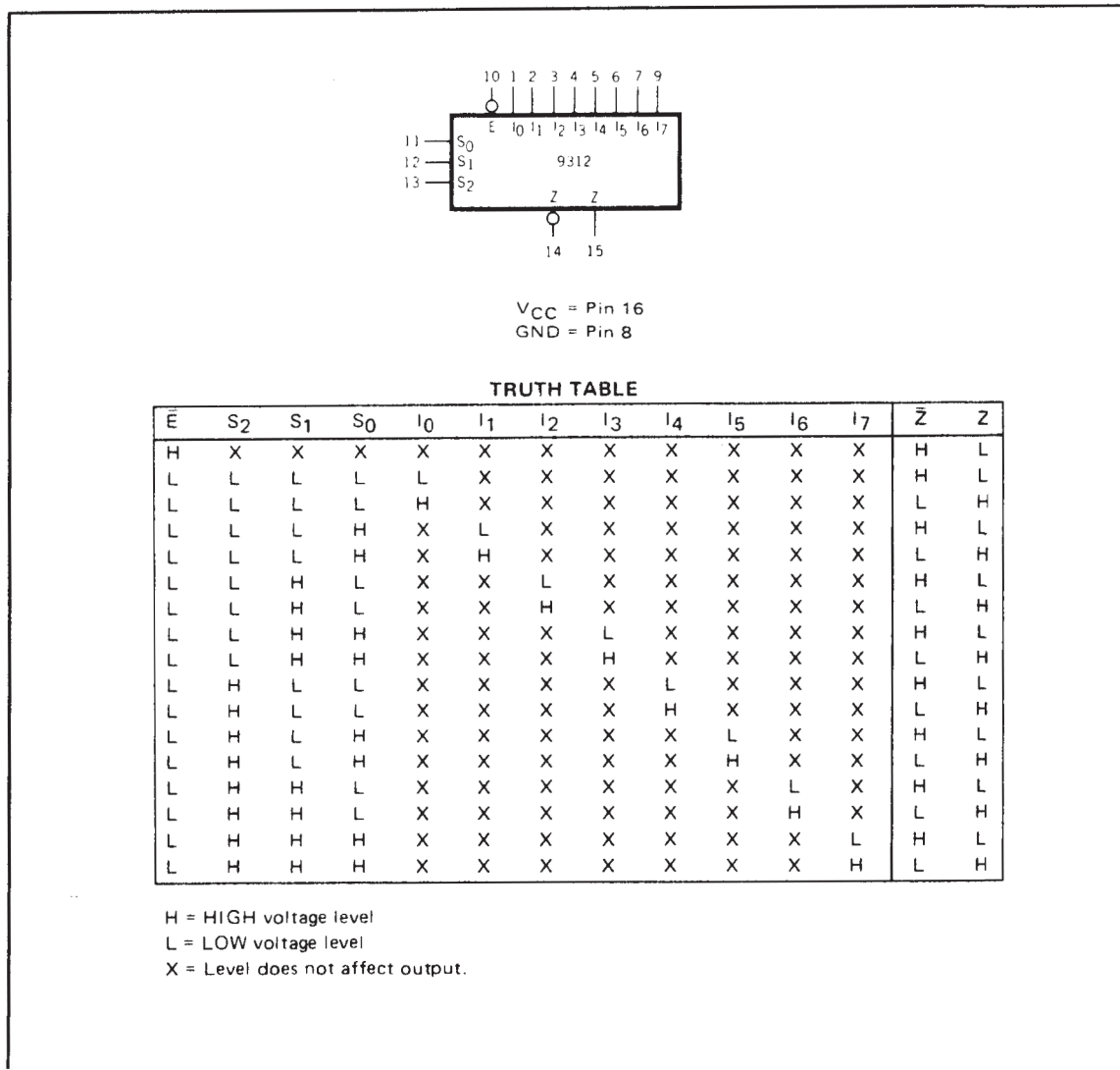
Figure 4-23. Eight-Input Multiplexer 1820-0615
