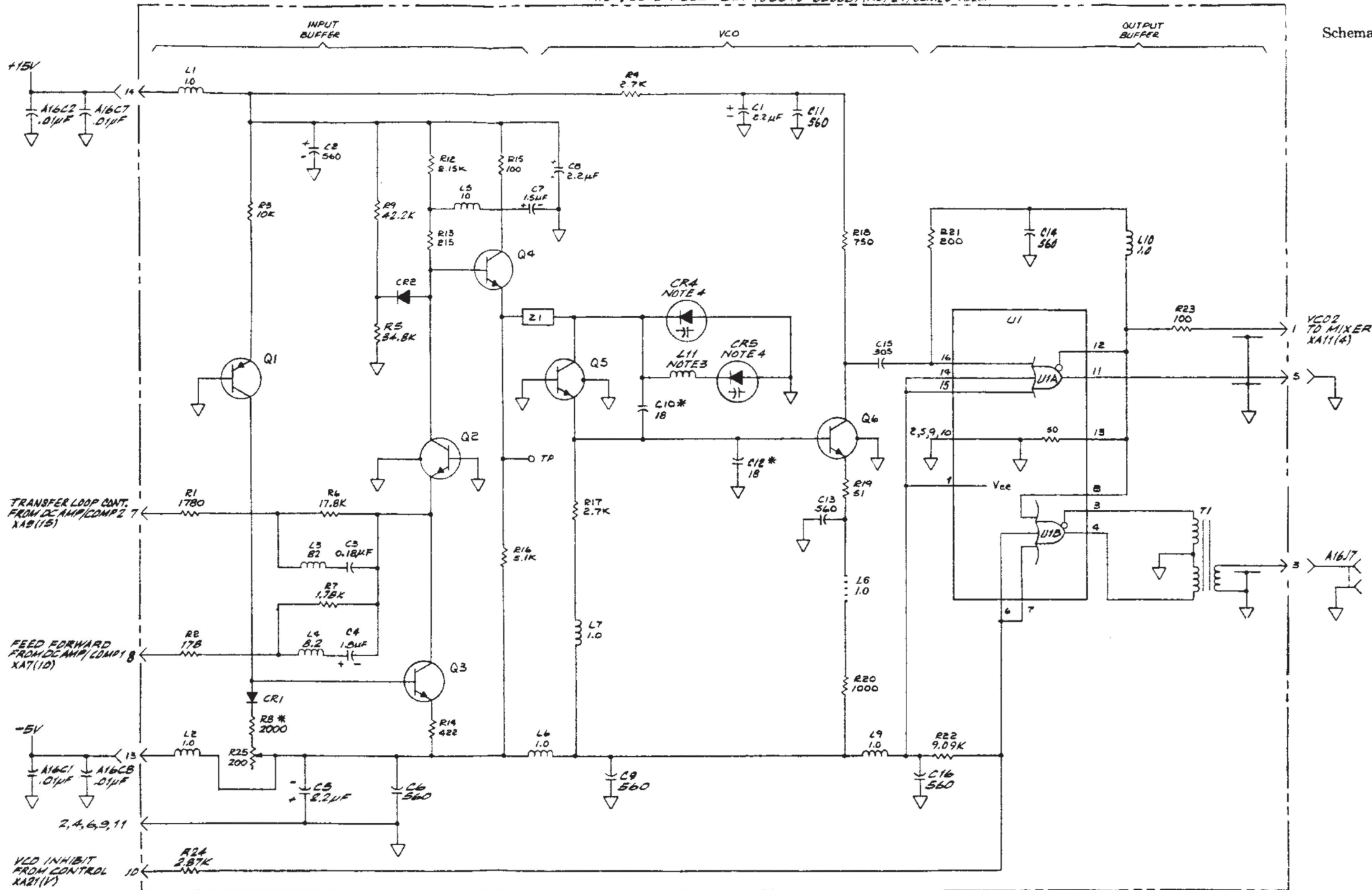
Figure 8-16. A10 VCO No. 2 Assembly
