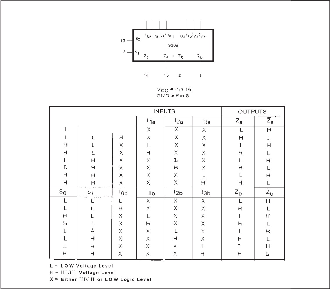
Figure 4-22. Four-Input Multiplexer 1820-0610
