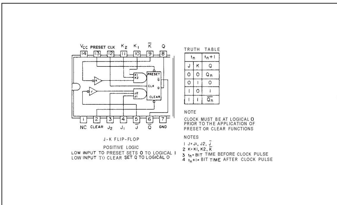
Figure 4-5. J-K Flip-Flop 1820-0065
