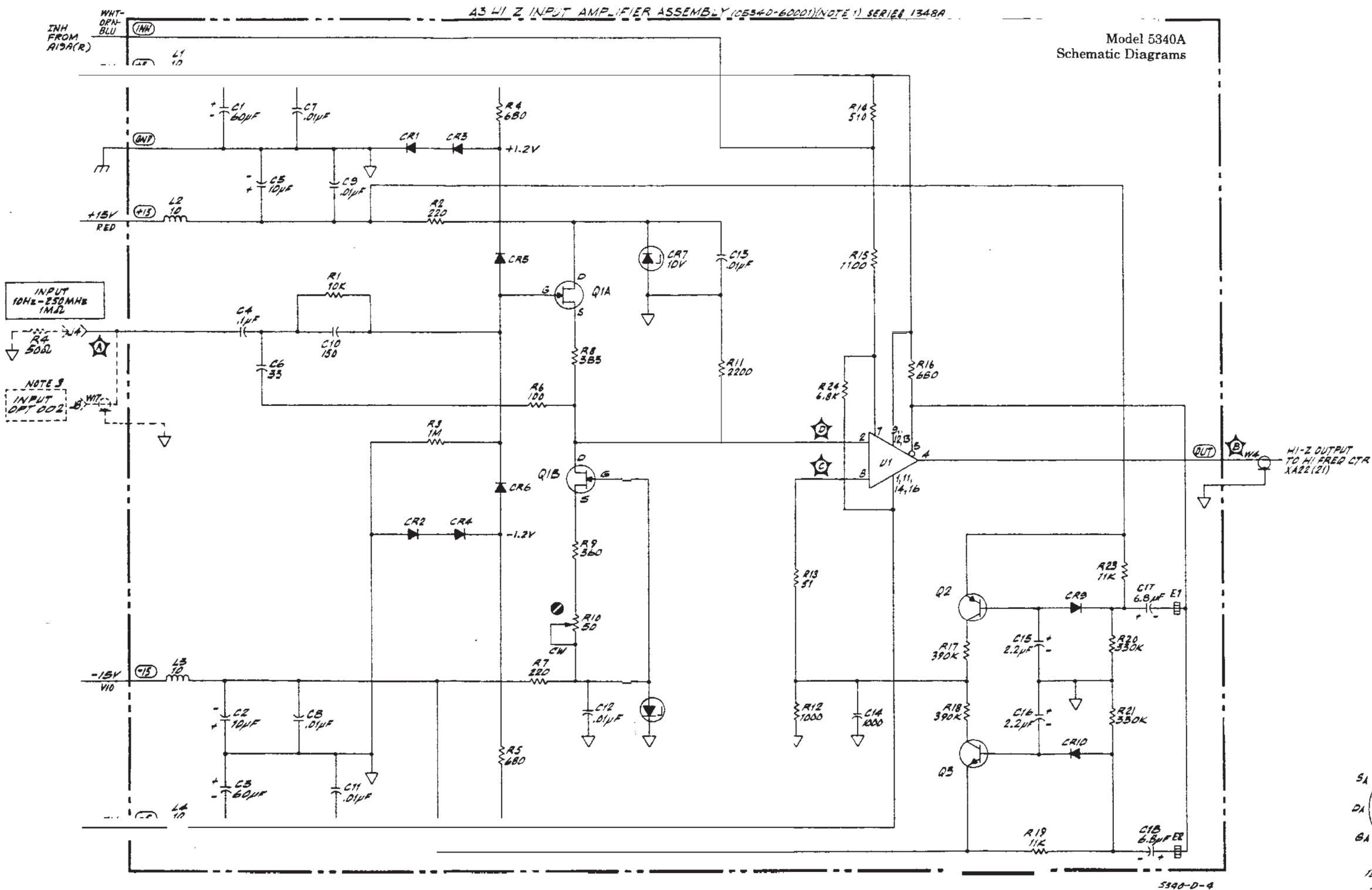
Figure 8-9. A3 HI-Z Input Amplifier Assembly
