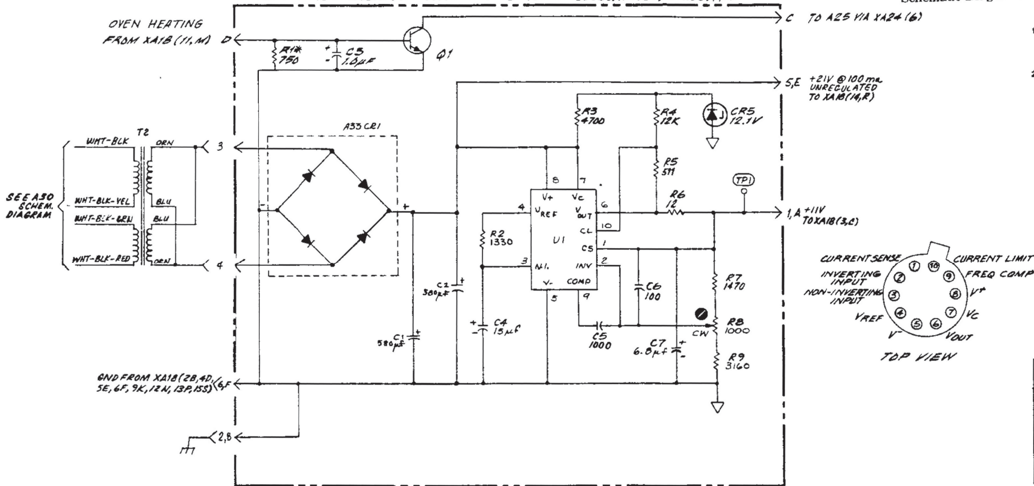
Figure 8-35. A33 Time Base Power Supply (Part f Option 001)
