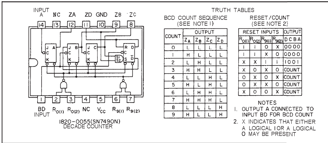
Figure 4-4. Decade Counter 1820-0055
