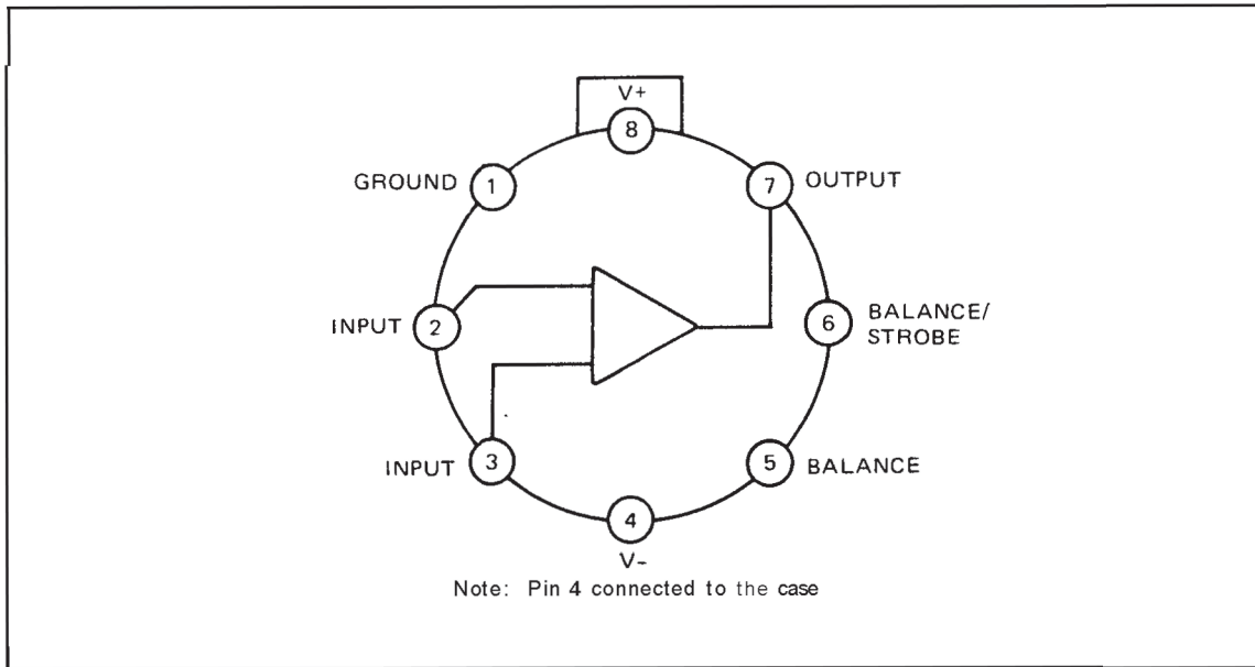
Figure 4-41. Voltage Comparator/Buffer 1826-0026
