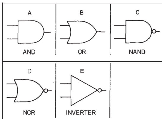
Figure 4-2. Gate Symbols
