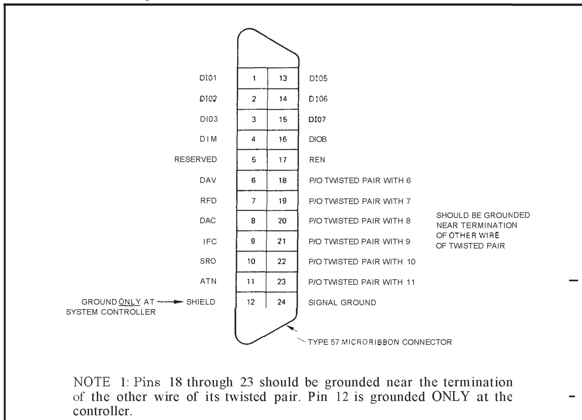
Figure 2-4. Pin Connections of the 10631A, B, C Cables
