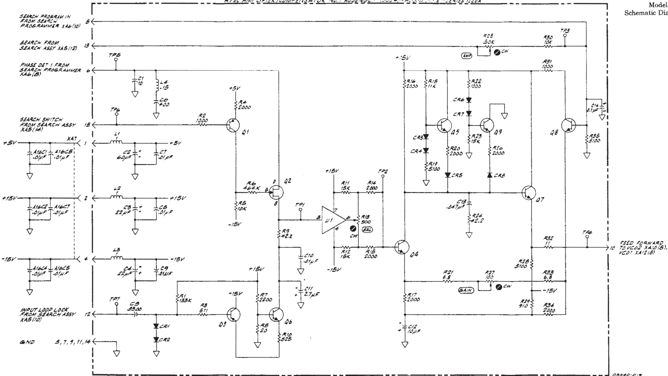
Figure 8-13. A7 DC Amplifier/Compensator No. 1 Assembly
