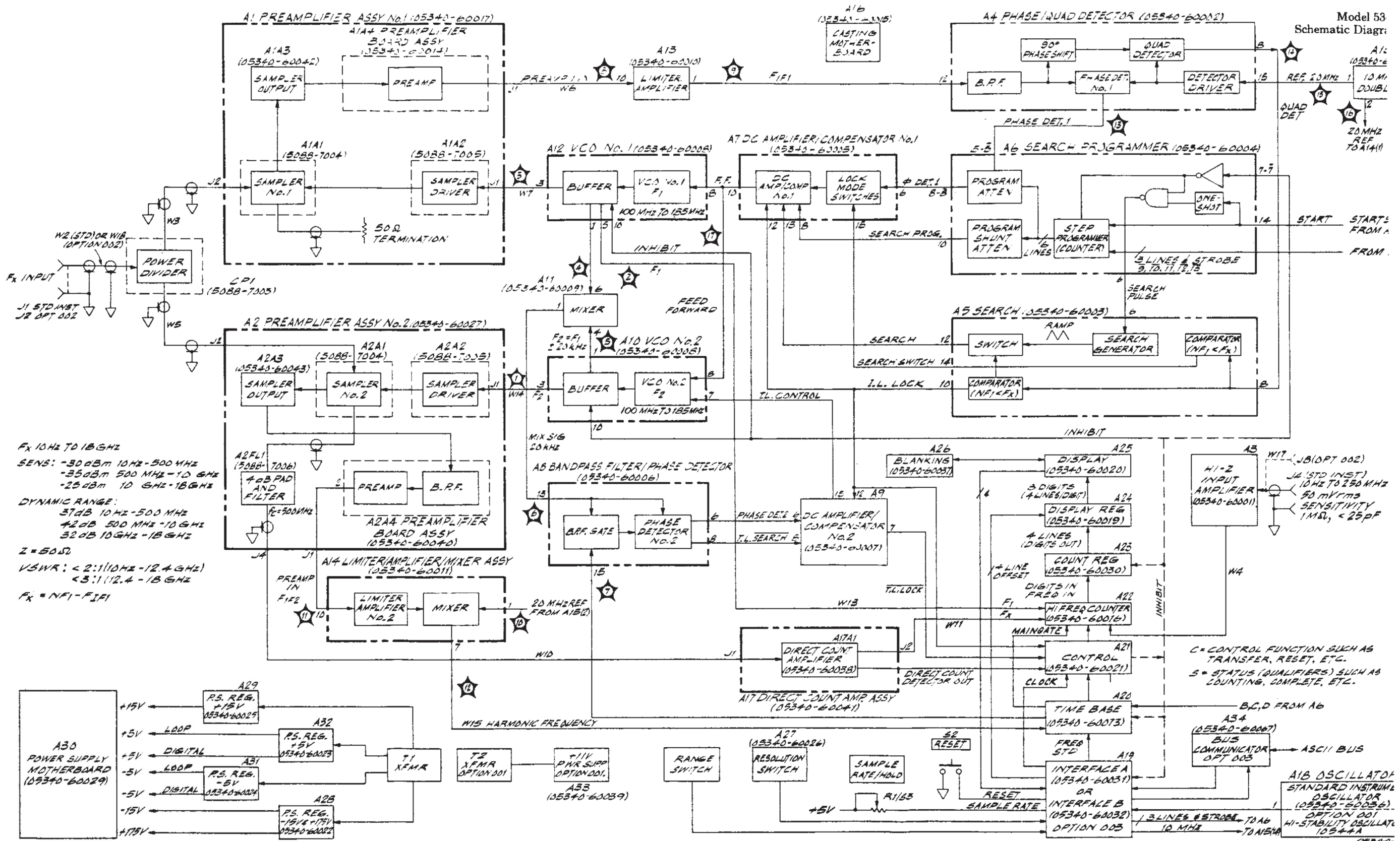
Figure 8-6. 5340A Block Diagram
