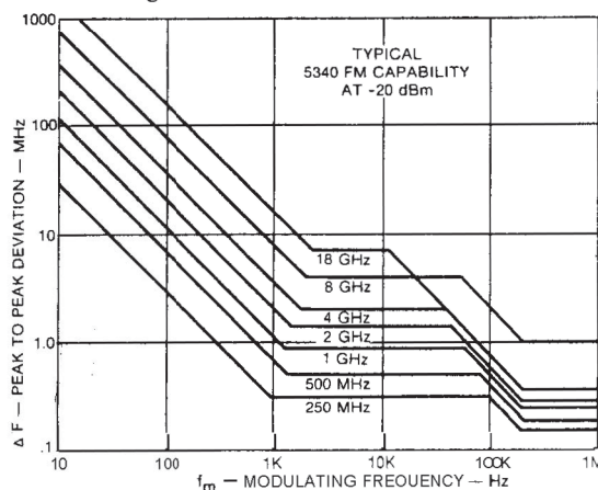
Figure 3-1. FM Characteristics
