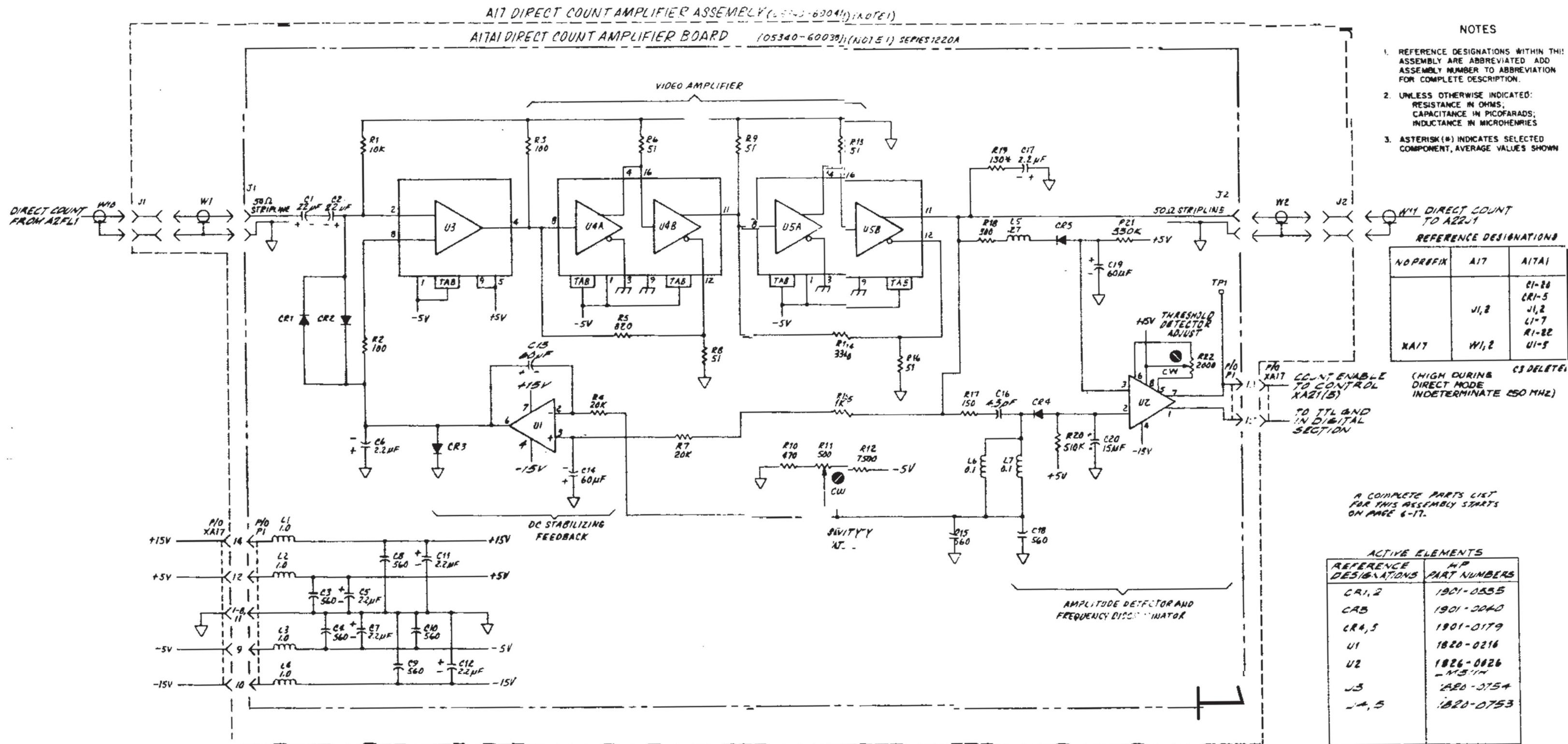
Figure 7-2. A17 Direct Count Amplifier Assembly (Series 1220A)
